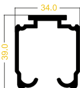
RIEL REF: T764
