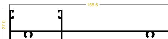
JAMBA TRES RIELES REF: 1731
