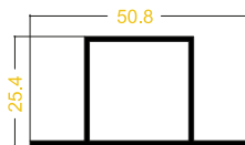
TUBULAR 1" X 1" DOBLE ALETA REF: T-078
