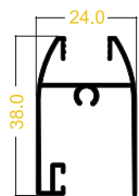
HORIZONTAL SUPERIOR CURVO REF: 874
